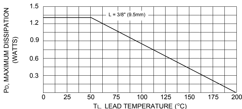
Fig. 1 POWER TEMPERATURE DERATING CURVE
