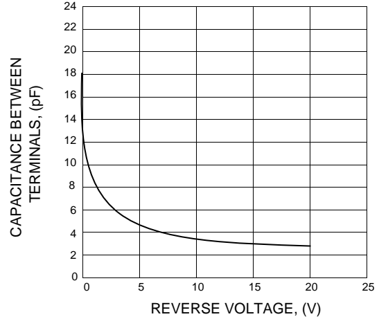
FIG.2 - CAPACITANCE BETWEEN TERMINALS CHARACTERISTICS
