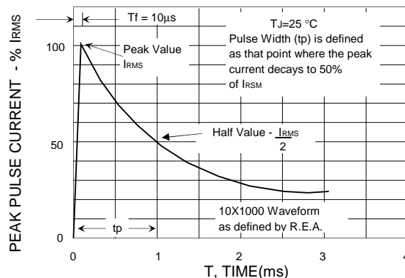
FIG.3 - PULSE WAVEFORM
