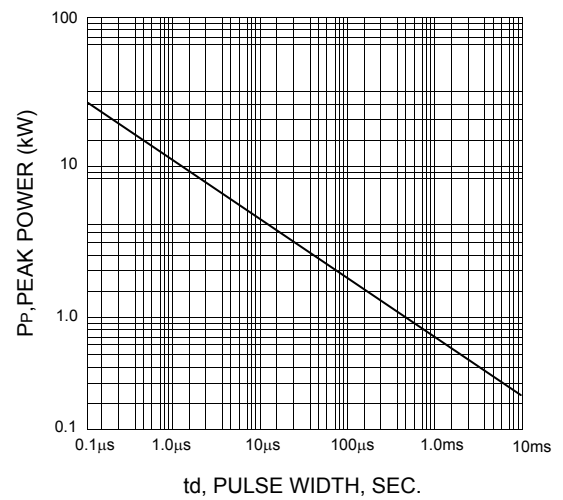
FIG.2 - PEAK PULSE POWER RATING CURVE
