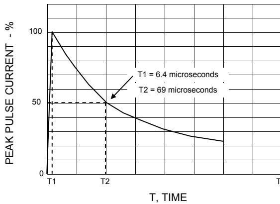
FIG.5 - PULSE WAVEFORM
