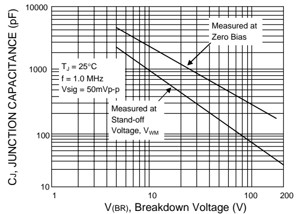
FIG. 6 - TYPICAL JUNCTION CAPACITANCE UNI-DIRECTIONAL
