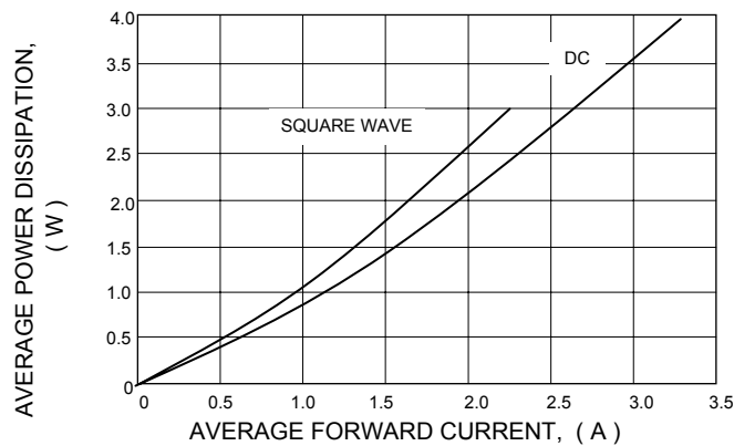
FIG. 5 - POWER DISSIPATION
