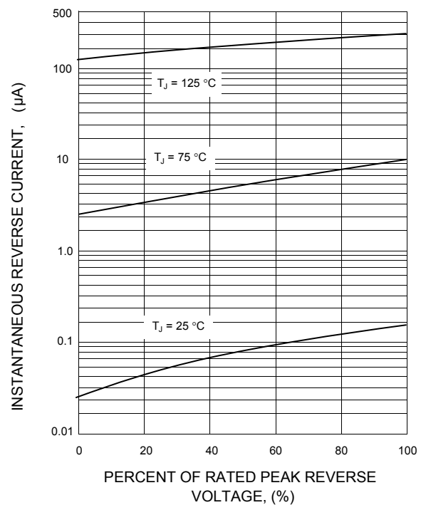
FIG. 4 - TYPICAL REVERSE CHARACTERISTICS PER LEG
