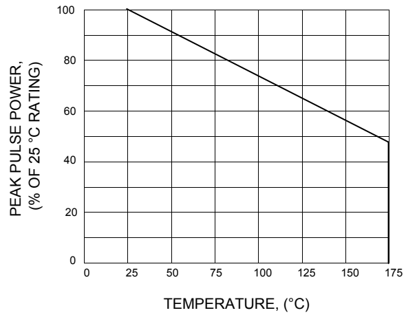
FIG.2 - DREATING CURVE
