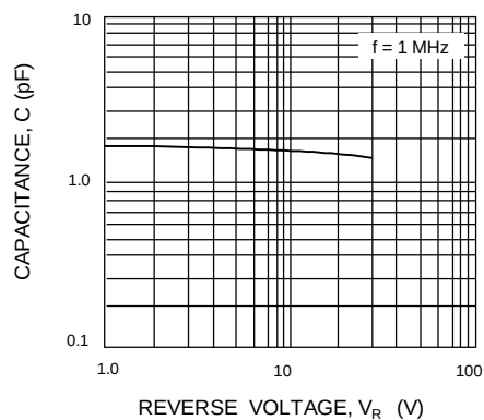
FIG.3 - CAPACITANCE Vs. REVERSE VOLTAGE
