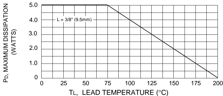
Fig. 1 POWER TEMPERATURE DERATING CURVE
