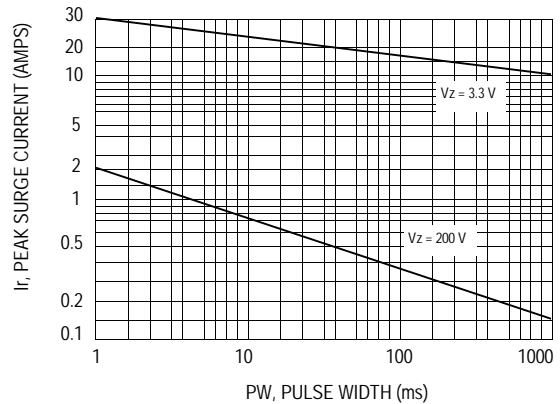
Fig. 4 Peak Surg Current versus Pulse Width
