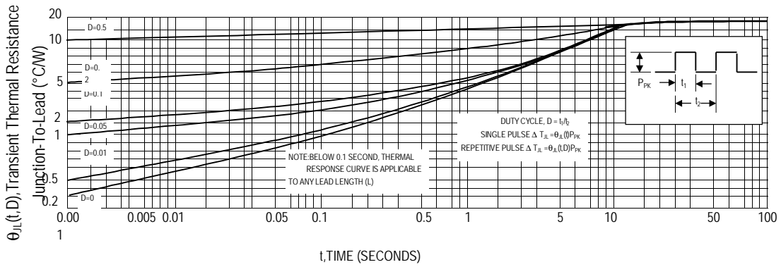
Fig 2. Typical Thermal Response L, Lead Length = 3/8 Inch
