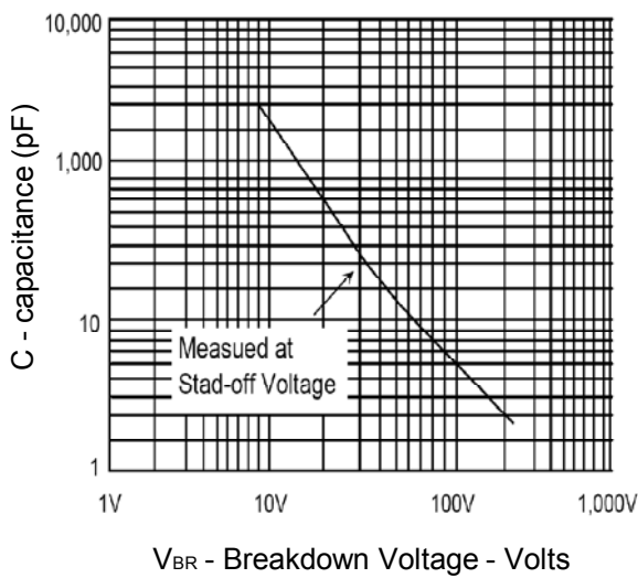
FIG.3 - TYPICAL CAPAITANCE VS. BREAKDOWN VOLTAGE
