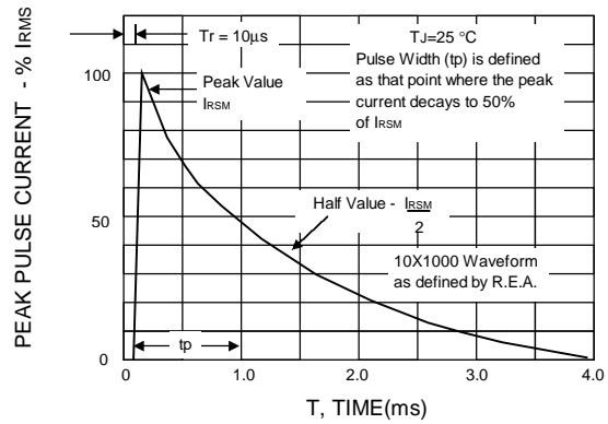
FIG.2 - PULSE WAVEFORM
